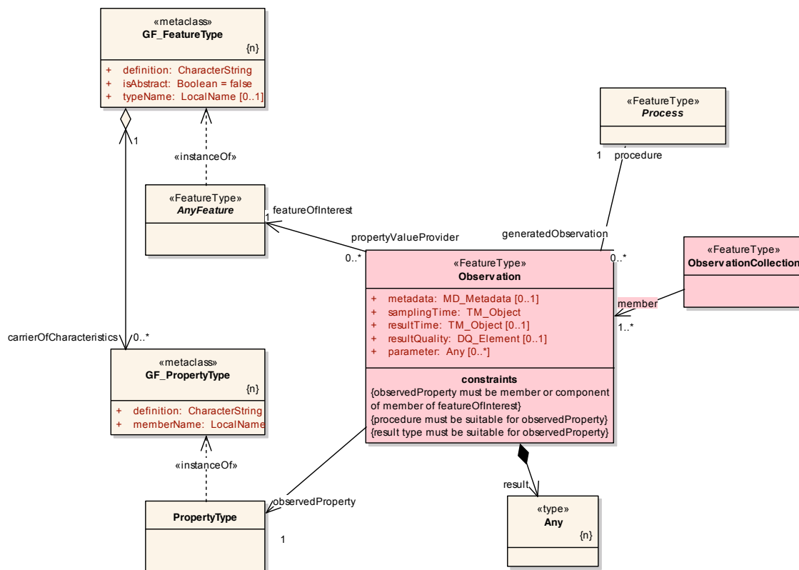
Figure 1. Summary of O & M model, taken from O G C 07-022
