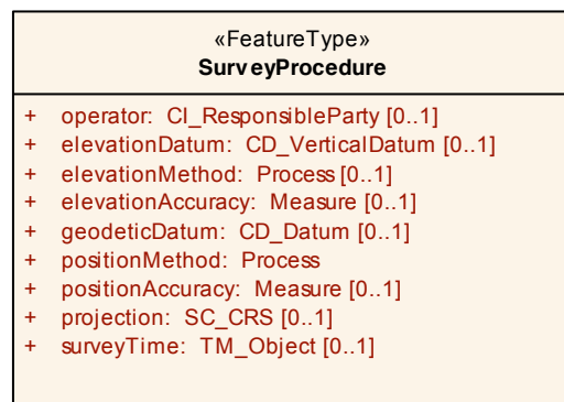
Figure 4. (Informative) Basic model for Survey Procedure
