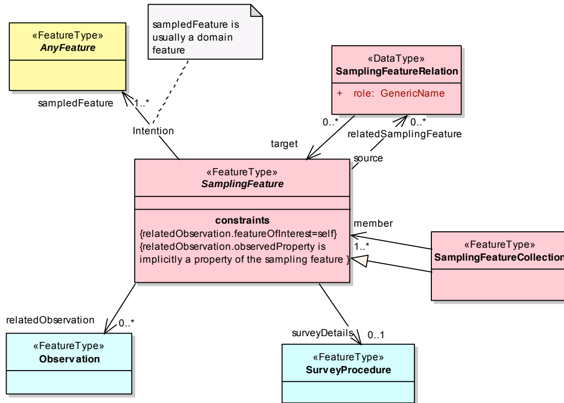
Figure 3. Basic model for sampling features
