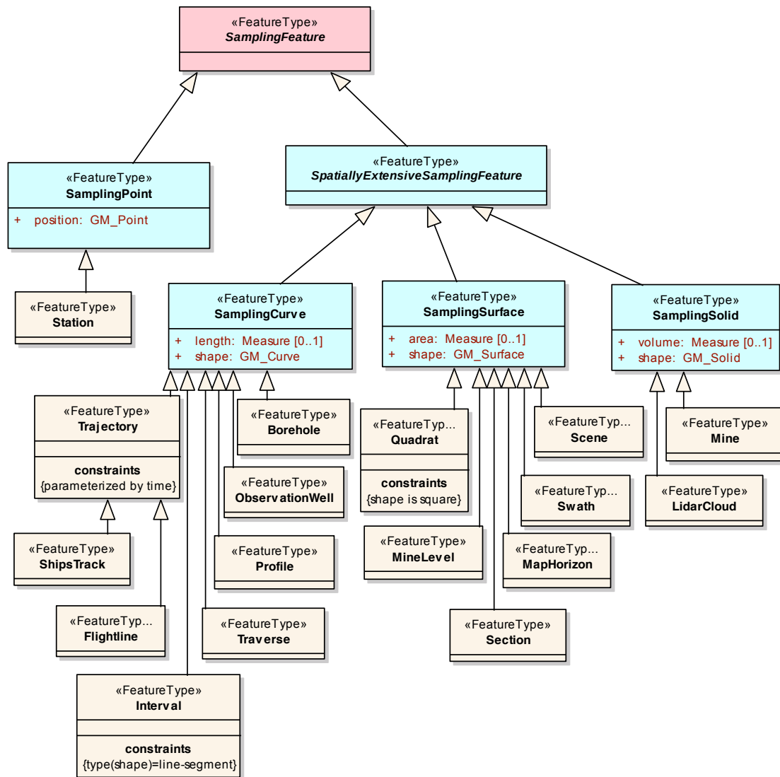
Figure 5. A hierarchy of types used for observation sampling.
